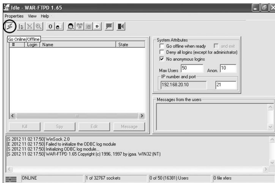
Figure 17-2: War-FTP 1.65 GUI
